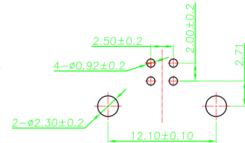
Recommnd PCB Layout
