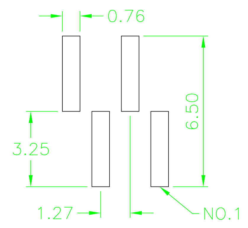
RECOMMENDED P.C.B SMT LAYOUT
